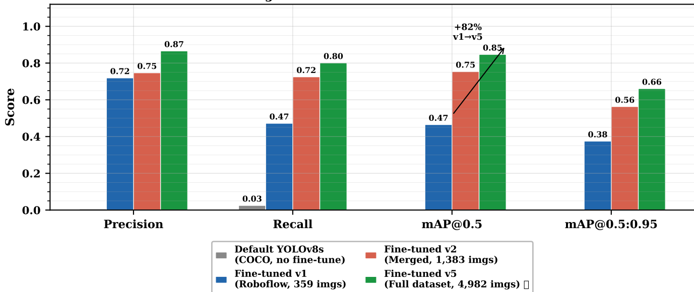
Model Performance Progression on Held-Out Test Set — Default → v1 → v2 → v5
